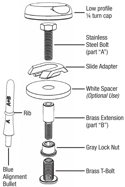
With Gray Lock Nut loosened, Insert Brass T-Bolt into toilet bolt slot.
