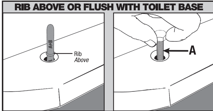
If Rib on Alignment Bullet is ABOVE toilet base, insert Stainless Steel Bolt (A) and start thread in Brass T-Bolt.
