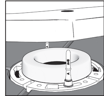
Add wax seal and set toilet using Alignment Bullets to position toilet. Apply body weight to help compress wax seal. Check location of Alignment Rib on Bullet before removing.
