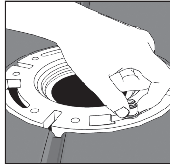
Center T-Bolt and hand tighten Gray Lock Nut.
