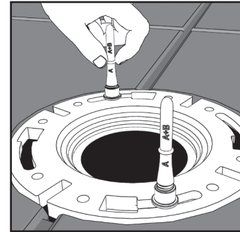
Insert Alignment Bullets into Brass T-Bolt Openings.
