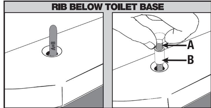
If the Rib on the Alignment Bullet is BELOW toilet base, thread Stainless Steel Bolt (A) into Brass Extension (B), and then thread in Brass T-Bolt.
